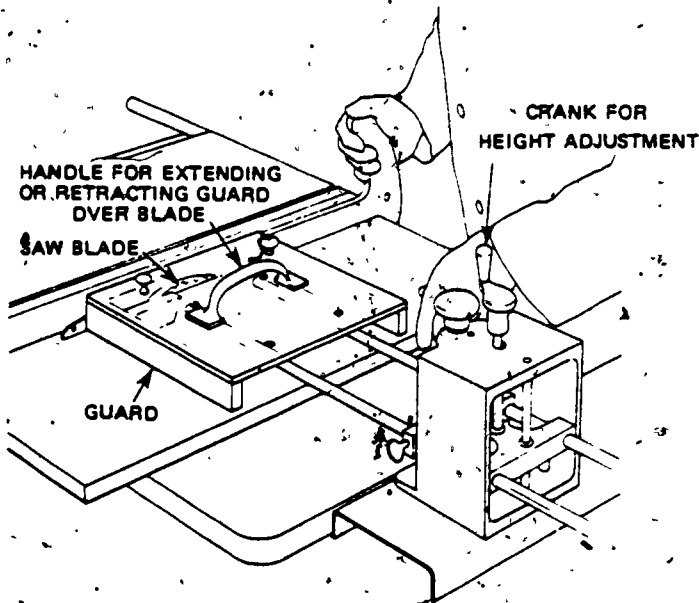
c. Adjustable guard on table saw.
