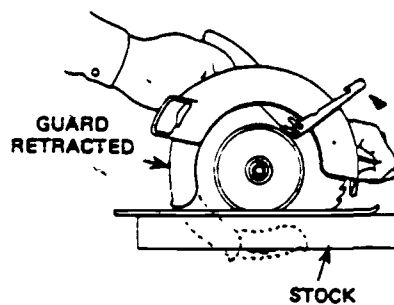
d. Self-adjusting guard on circular saw.
