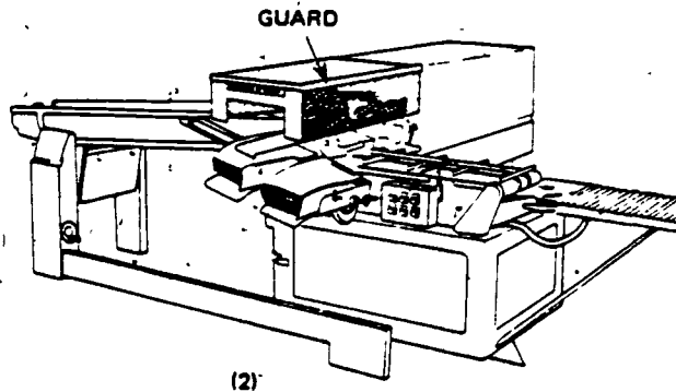
b. Interlocking guards on (1) corn cutter and (2) automatic bread bagging machine.
